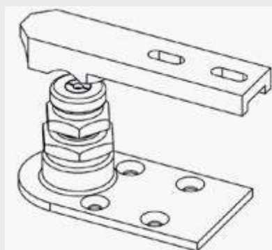
Floor Pivot
